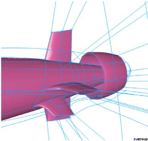
Engineers at NSWC used Gridgen to make this block structure around a submarine propulsor.
