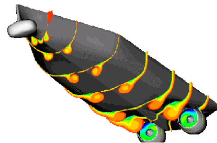
Vortices shed from the sonar dome of this surface ship travel under the hull and into the propulsors.
