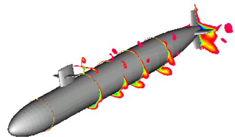
The asymmetric vortices shed from the sail of this submarine show the effects of pitch and yaw.
